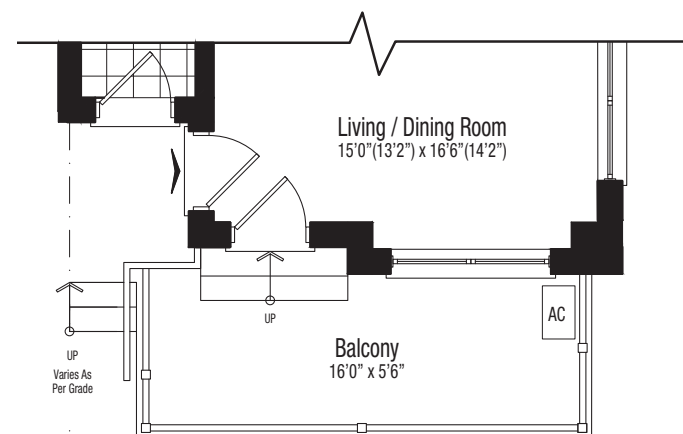
PART. SF(E3W) ENTRY LEVEL
