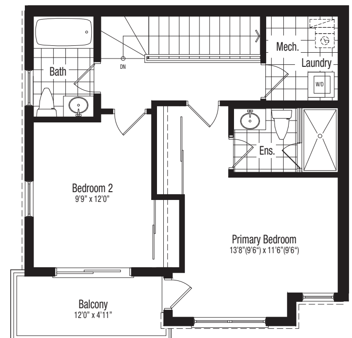
S2(E) - THIRD LEVEL
