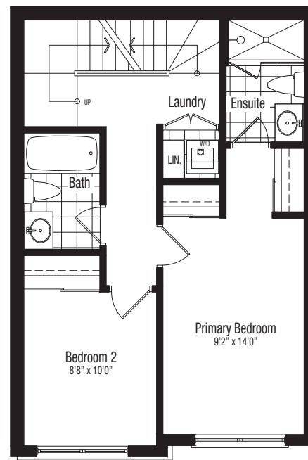
SG - FOURTH LEVEL
