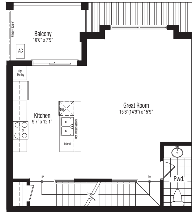
S3 - SECOND LEVEL
